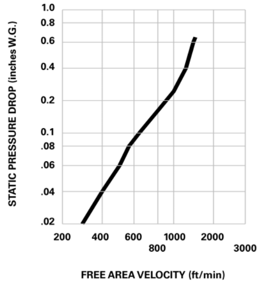
V3 - VERTICAL LOUVER with 1-inch recessing flange
