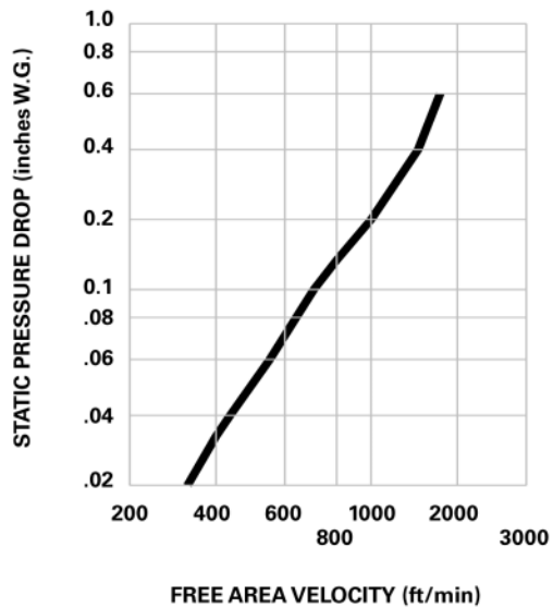
H2 - HORIZONTAL LOUVER with 1-inch recessing flange
