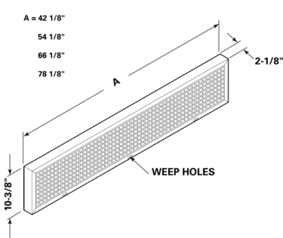
V2 - VERTICAL LOUVER with Lattice
