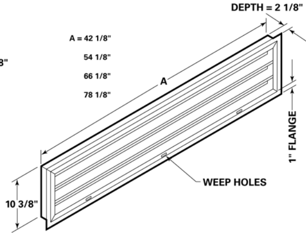
H2 - HORIZONTAL LOUVER with 1-inch recessing flange
