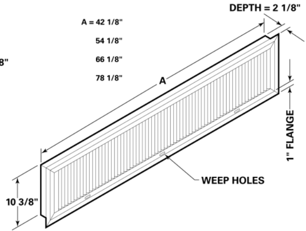
V3 - VERTICAL LOUVER with 1-inch recessing flange
